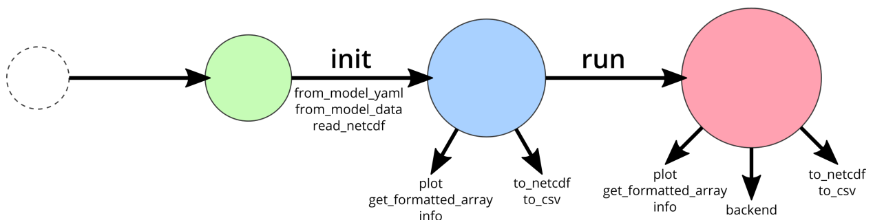
Fig. 17: Representation of the Calliope Model object, growing from an empty class to having methods to view, plot and save data, and to interface with the solver backend.
